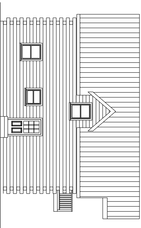
LEFT SIDE ELEVATION SCALE: 1/4"=1'-0"
